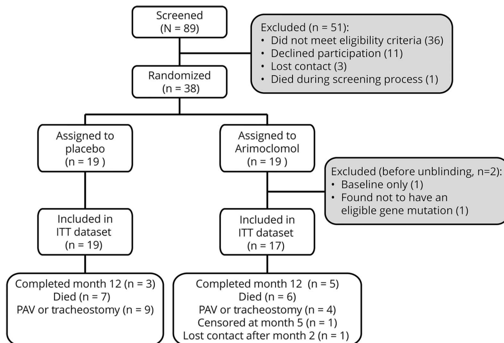
Figure 1 Consort diagram
